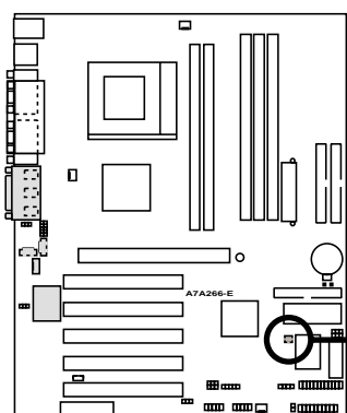
A7A266-E Wake-On-Ring Connector
